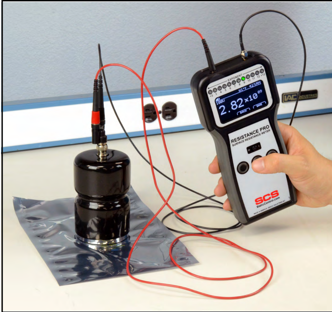
Figure 2. Using the Concentric Ring Probe with the SCS 770760 Resistance Pro Meter
